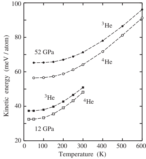
Figure 4. Temperature dependence of the kinetic energy of hcp solid helium at two different pressures, as derived from PIMC simulations: P = 12 GPa (squares) and 52 GPa (circles). Open and filled symbols correspond to ^4\text{He} and ^3\text{He} , respectively. Error bars of the simulation results are less than the symbol size. The dashed lines are guides to the eye.
