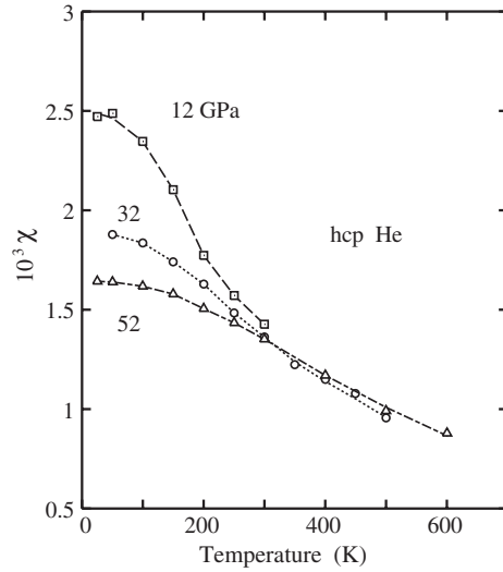
Figure 3. Isotopic effect on the lattice parameter a of hcp helium, as obtained from PIMC simulations. Shown is the parameter \chi = (a_3 - a_4)/a_4 as a function of temperature for three different pressures: squares, 12 GPa; circles, 32 GPa; triangles, 52 GPa. Error bars are of the order of the symbol size. The lines are guides to the eye.
