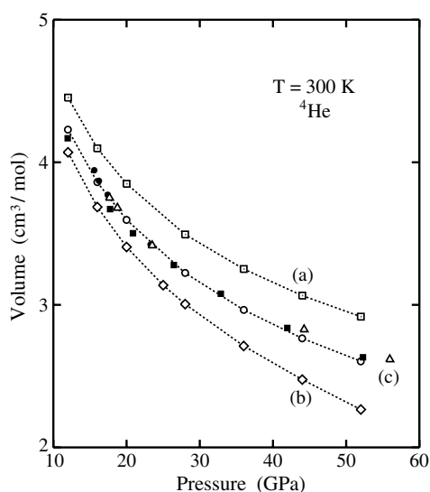
Figure 1. Equation of state pressure–volume of hcp ^4\text{He} at 300 K, as derived from PIMC simulations for different interatomic potentials. (a) Open squares: only two-body interactions with an Aziz-type potential [27]; (b) open diamonds: two-body terms as in [27] and three-body interactions, as defined in [29]; (c) open circles: same potential as (b), but with the exchange three-body interaction rescaled by 2/3 . Error bars of the simulation results are less than the symbol size. Dotted lines are guides to the eye. Open triangles show earlier results obtained from PIMC simulations in the NVT ensemble [17], with the attractive exchange interaction rescaled as in (c). Black symbols show experimental data obtained by Mao et al [3] (filled circles) and Loubeyre et al [4] (filled squares).
