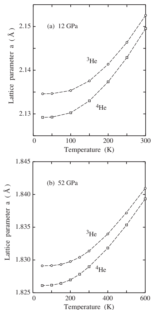
Figure 2. Temperature dependence of the lattice parameter a of hcp helium, derived from PIMC simulations at two different pressures: (a) 12 GPa and (b) 52 GPa. Squares and circles indicate results for ^4\text{He} and ^3\text{He} , respectively. Error bars are smaller than the symbol size. Dashed lines are guides to the eye.
