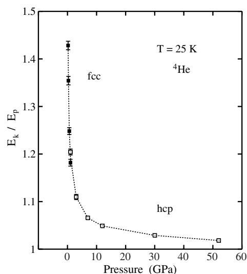
Figure 5. Kinetic-to-potential energy ratio, E_k/E_p , for solid ^4\text{He} as a function of applied pressure at T = 25 K. Black and open symbols correspond to fcc and hcp phases, respectively. Error bars, where not shown, are smaller than the symbol size.
